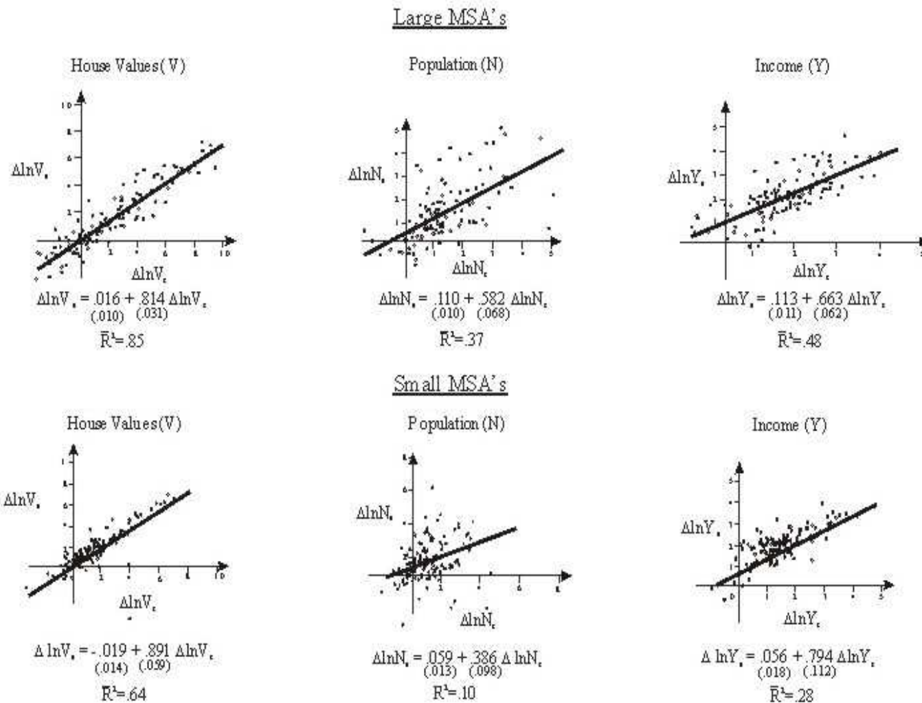
Figure 1: City-Suburban Growth Correlations
